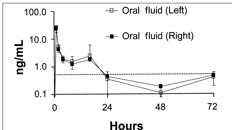
Figure 1. Mean THC concentrations by GC-MS-MS in oral fluid specimens collected simultaneously from the left and right sides of the oral cavity of 10 subjects following smoking of a single marijuana cigarette (Study 1). Error bars represent standard error of the mean. The dotted line indicates the cutoff concentration (0.5 ng/mL) used to designate positive specimens in this assay.
