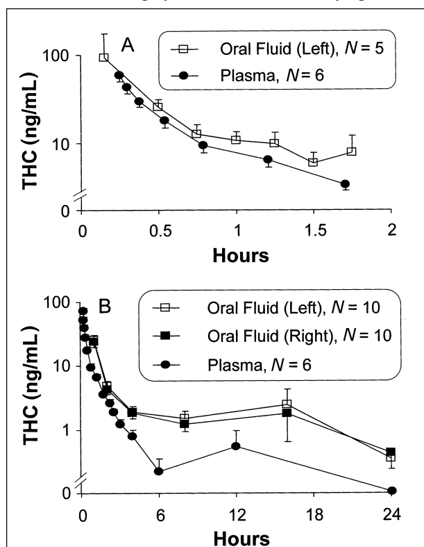
Figure 6. Comparison of THC in oral fluid and plasma (17) over short (A) and long (B) timecourses following marijuana smoking. Panel A illustrates THC in oral fluid of Study 2 (current study) following smoking of a single marijuana cigarette (20–25 mg of THC) by 5 male subjects compared to THC in plasma (17) following smoking of a single marijuana cigarette (15.8 mg of THC) by 6 male subjects. Panel B illustrates THC in oral fluid of Study 1 (current study) following smoking of a single marijuana cigarette (20–25 mg of THC) by 10 male subjects compared to THC in plasma following smoking of a single marijuana cigarette (15.8 mg of THC) by 6 male subjects. Error bars represent standard error of the mean (SEM).
